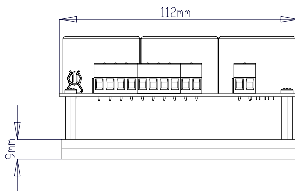
Figure 2-4: PS1 - Side View, Width
