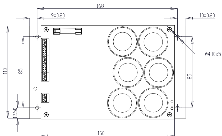
Figure 2-2: PS1 - Top View
