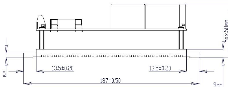
Figure 2-3: PS1 - Side View, Length
